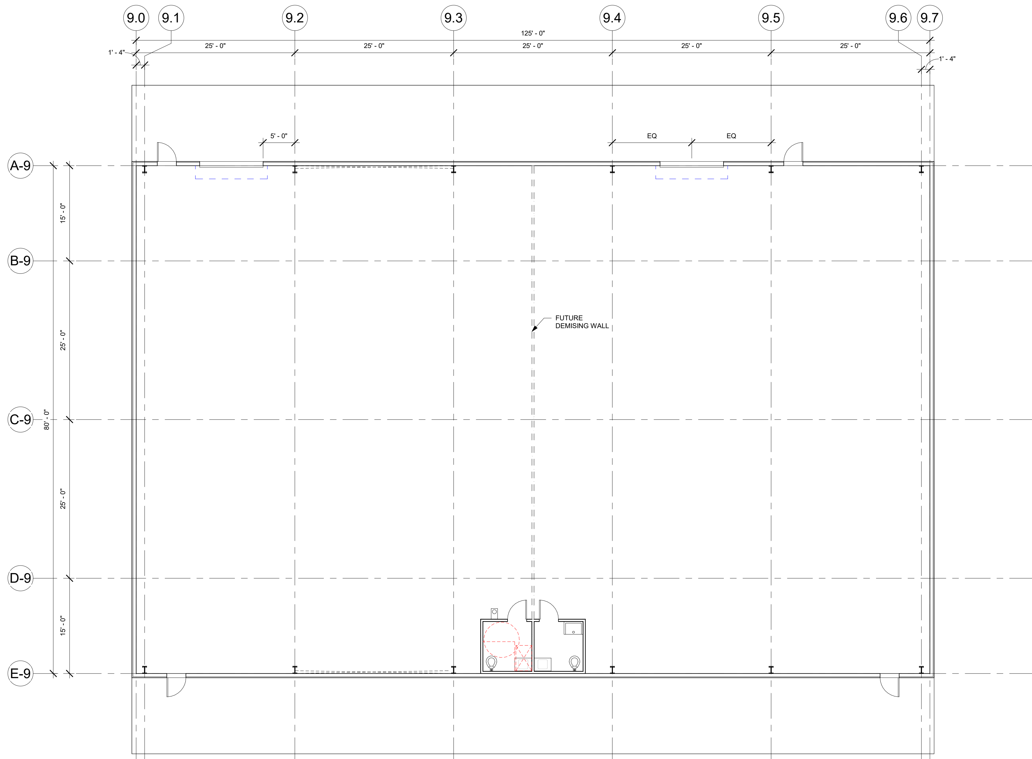
1 BUILDING 9 - FLOOR PLAN 1/8" = 1'-0"
