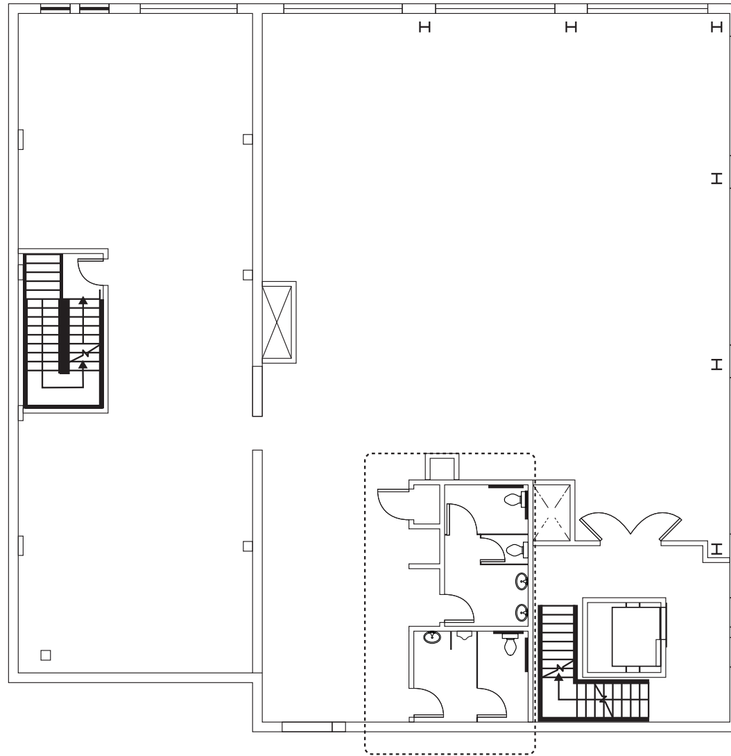
LEVEL 2 FLOOR PLAN
