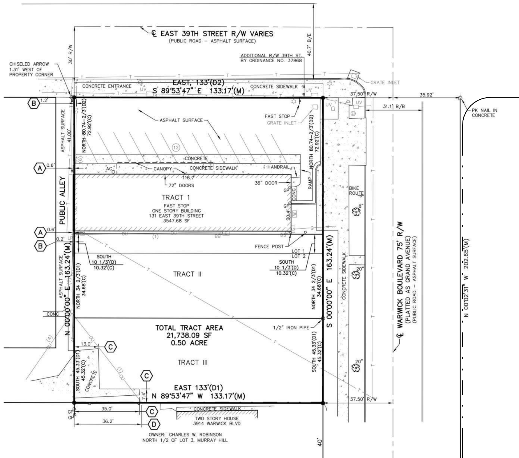
1 SITE PLAN 1" = 30'-0"
