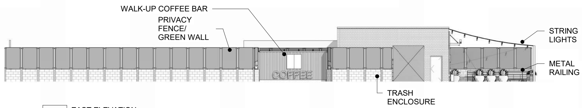
2 EAST ELEVATION 1/16" = 1'-0"
