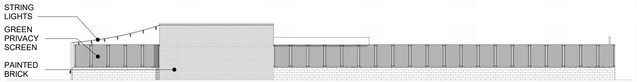
1 WEST ELEVATION 1/16" = 1'-0"
