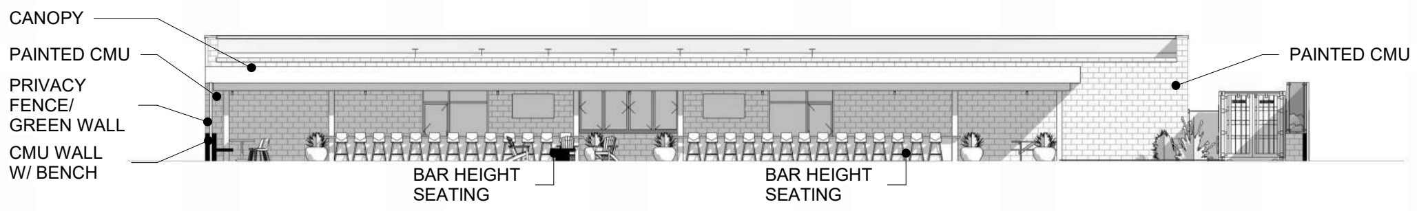
3 SOUTH ELEVATION 1/16" = 1'-0"
