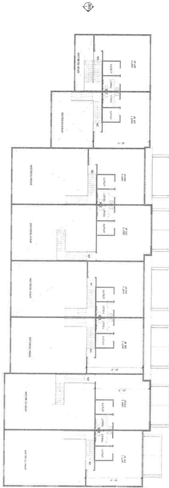
SECOND FLOOR PLAN 1/8" = 1'-0"
