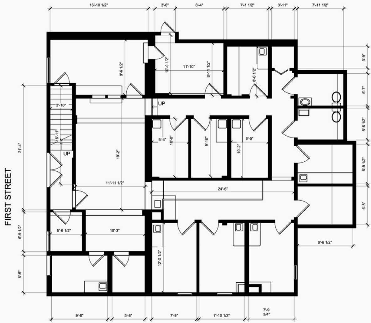
10 FIRST STREET, HACKENSACK, NJ GROUND FLOOR
