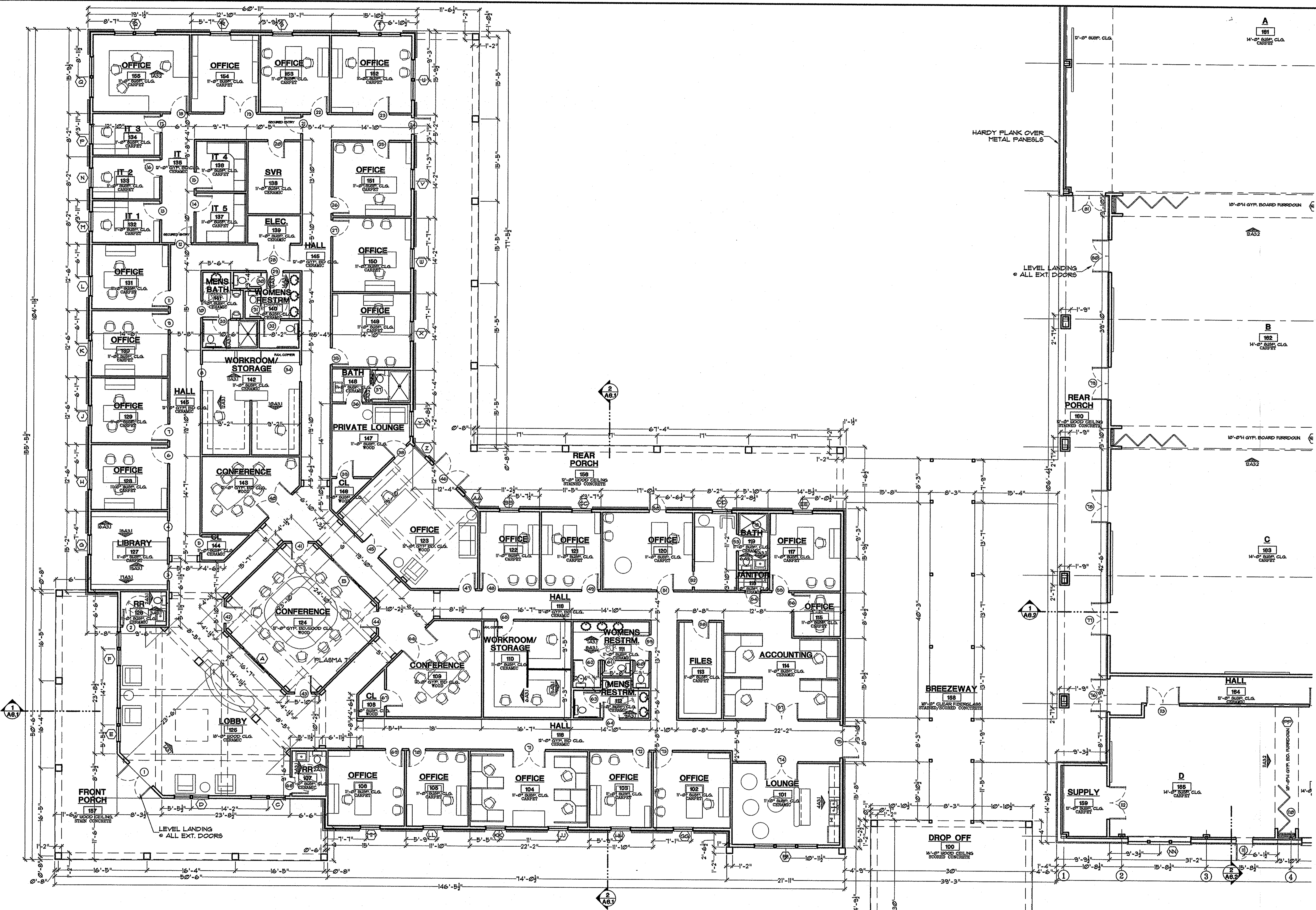
OFFICE BLDG. 1 FLOOR PLAN 1/8" = 1'-0"
