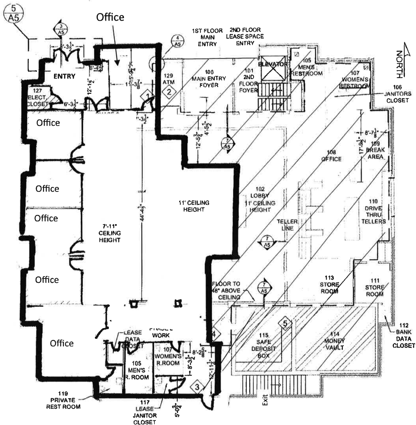
FLOOR PLAN 1/8" SCALE
