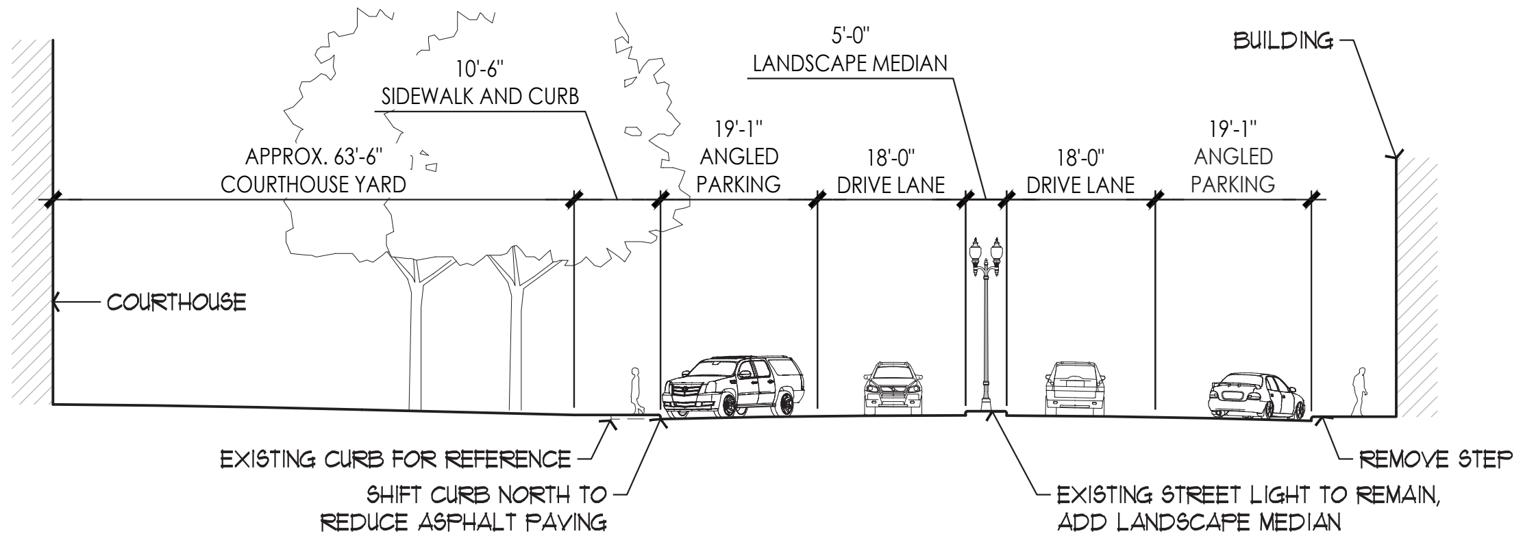
PROPOSED LAYOUT
