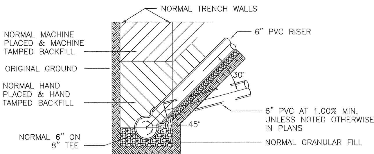
TEE ORIENTATION AND RISER DETAIL N.T.S.
