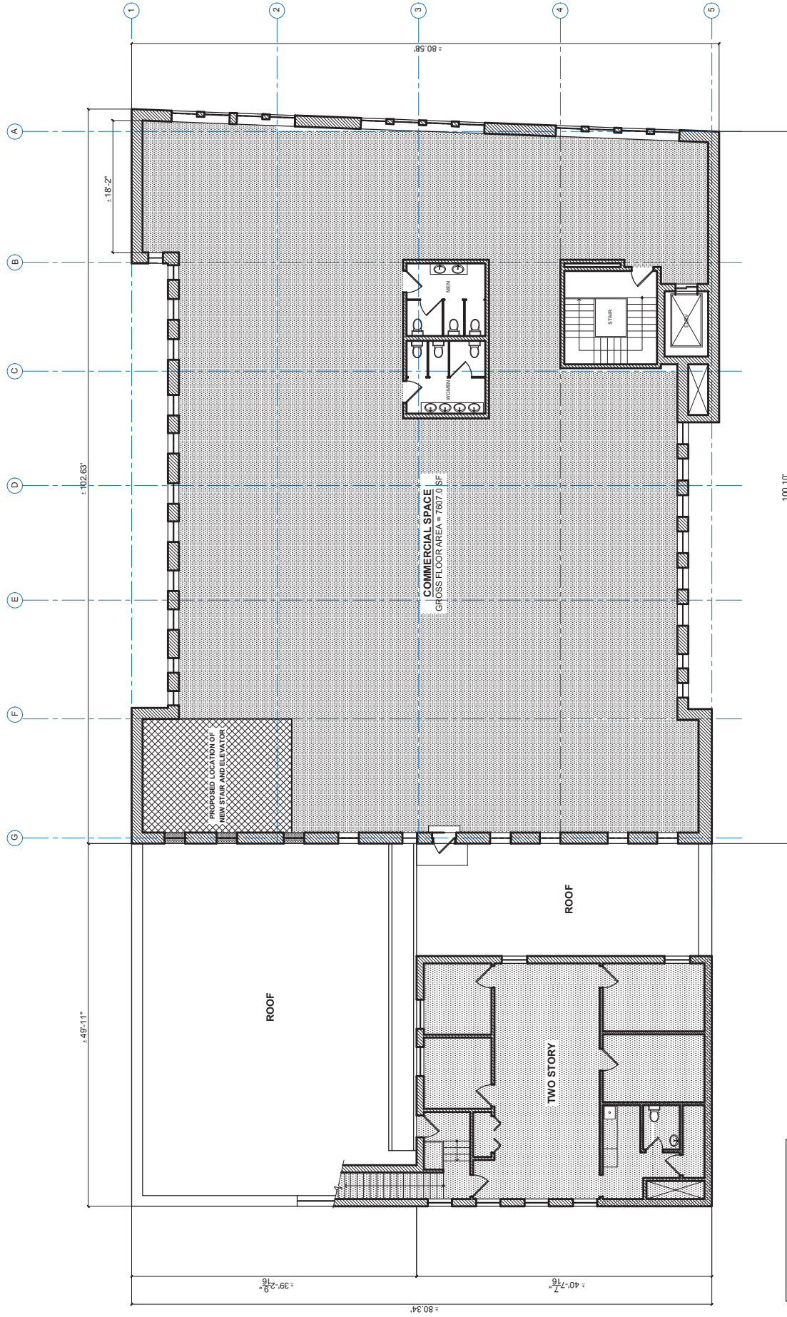
1 | A-1 | SECOND FLOOR PLAN (EXISTING) GROSS FLOOR AREA=7607.0 S.F.
