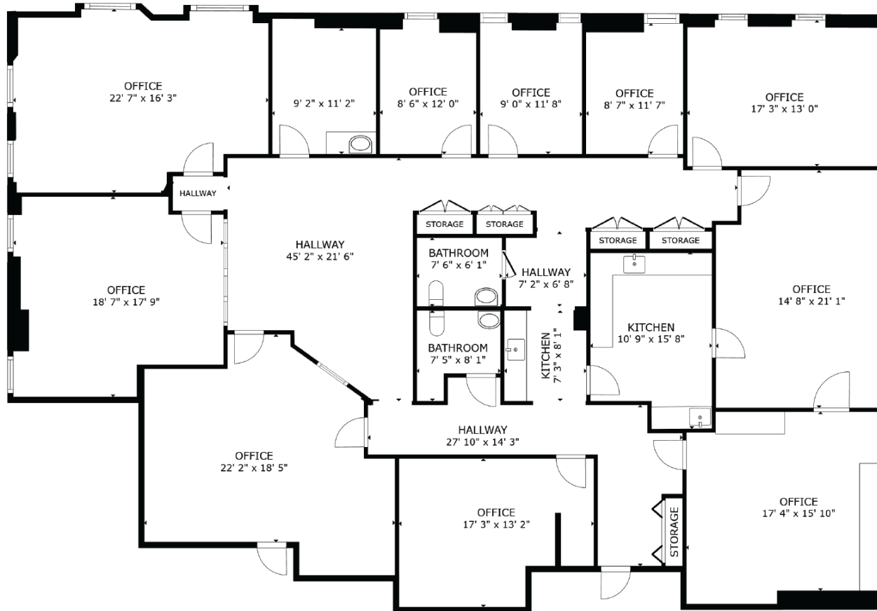
KEY PLAN
