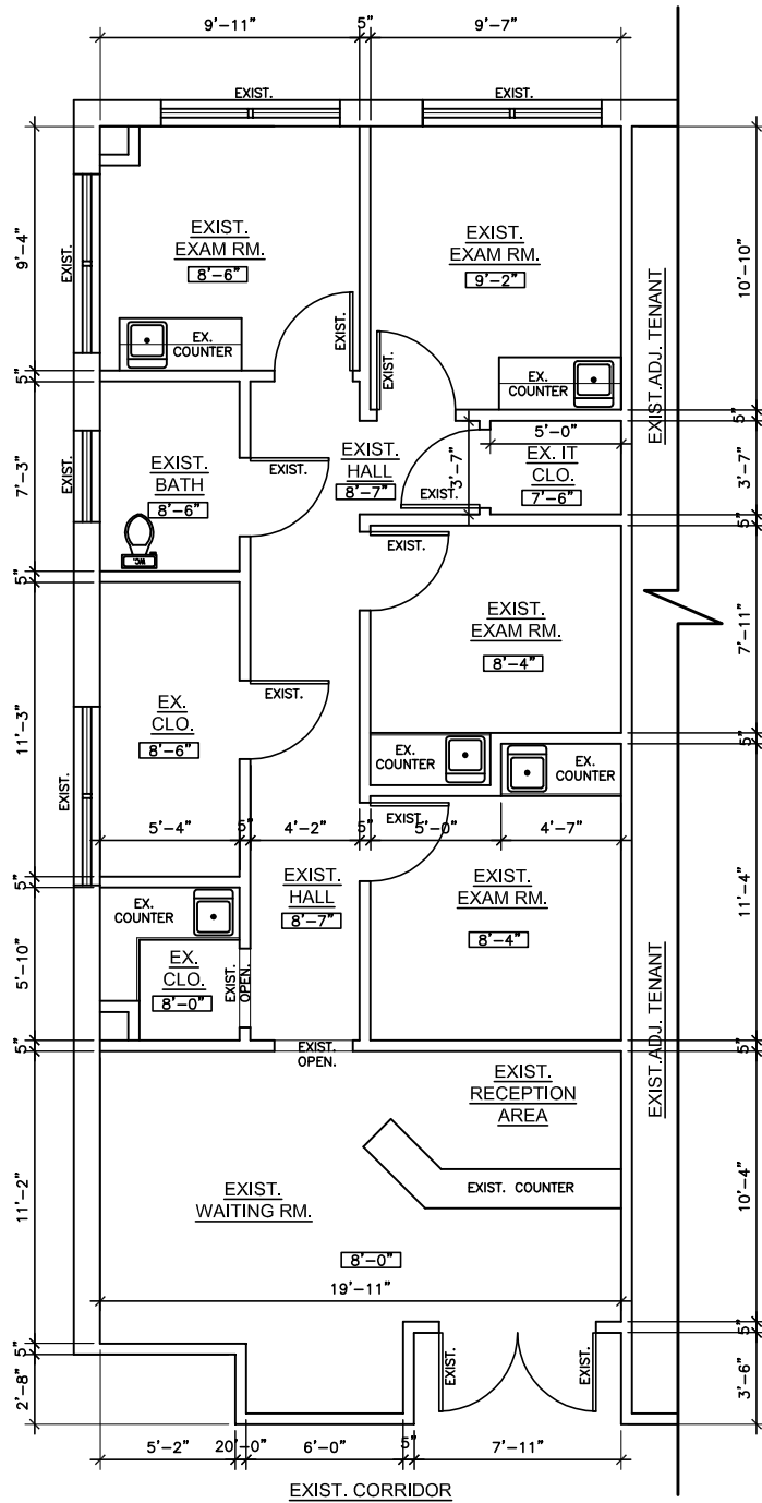
1 EXIST. FLOOR PLAN SCALE: 1/8" = 1'-0"
