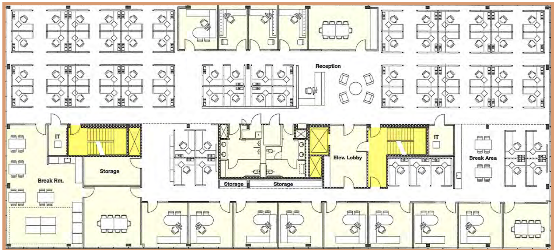
HYPOTHETICAL PLAN
