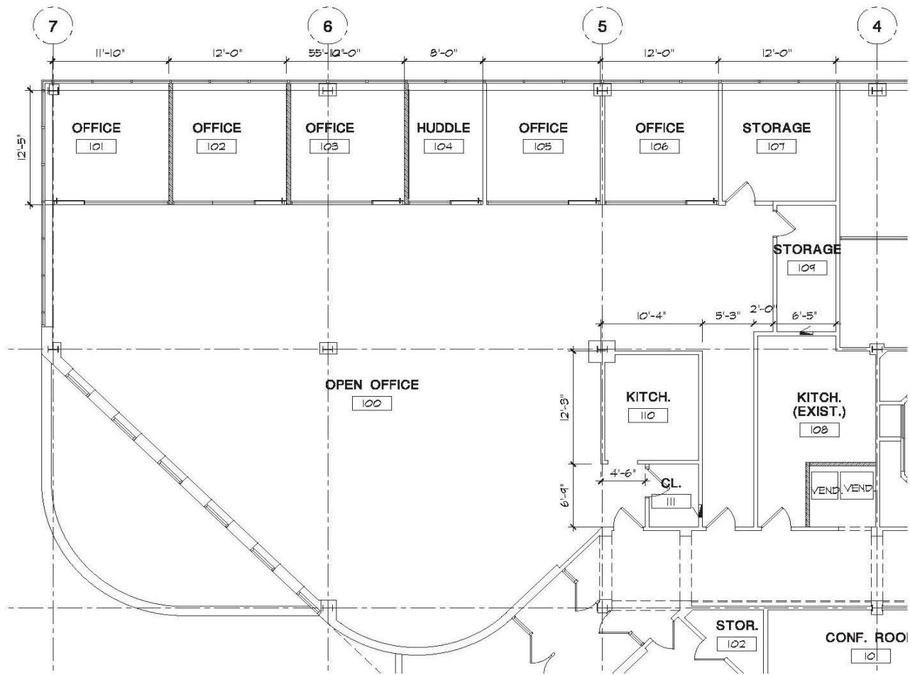
1ST FLOOR - FLOOR PLAN 1/4" = 1'-0"
