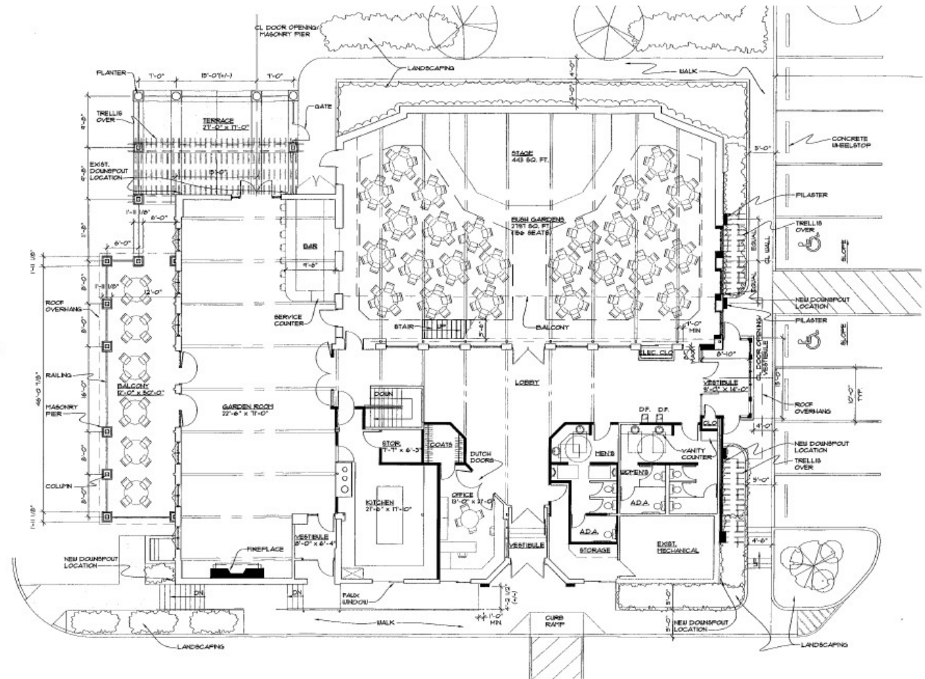
First Floor
