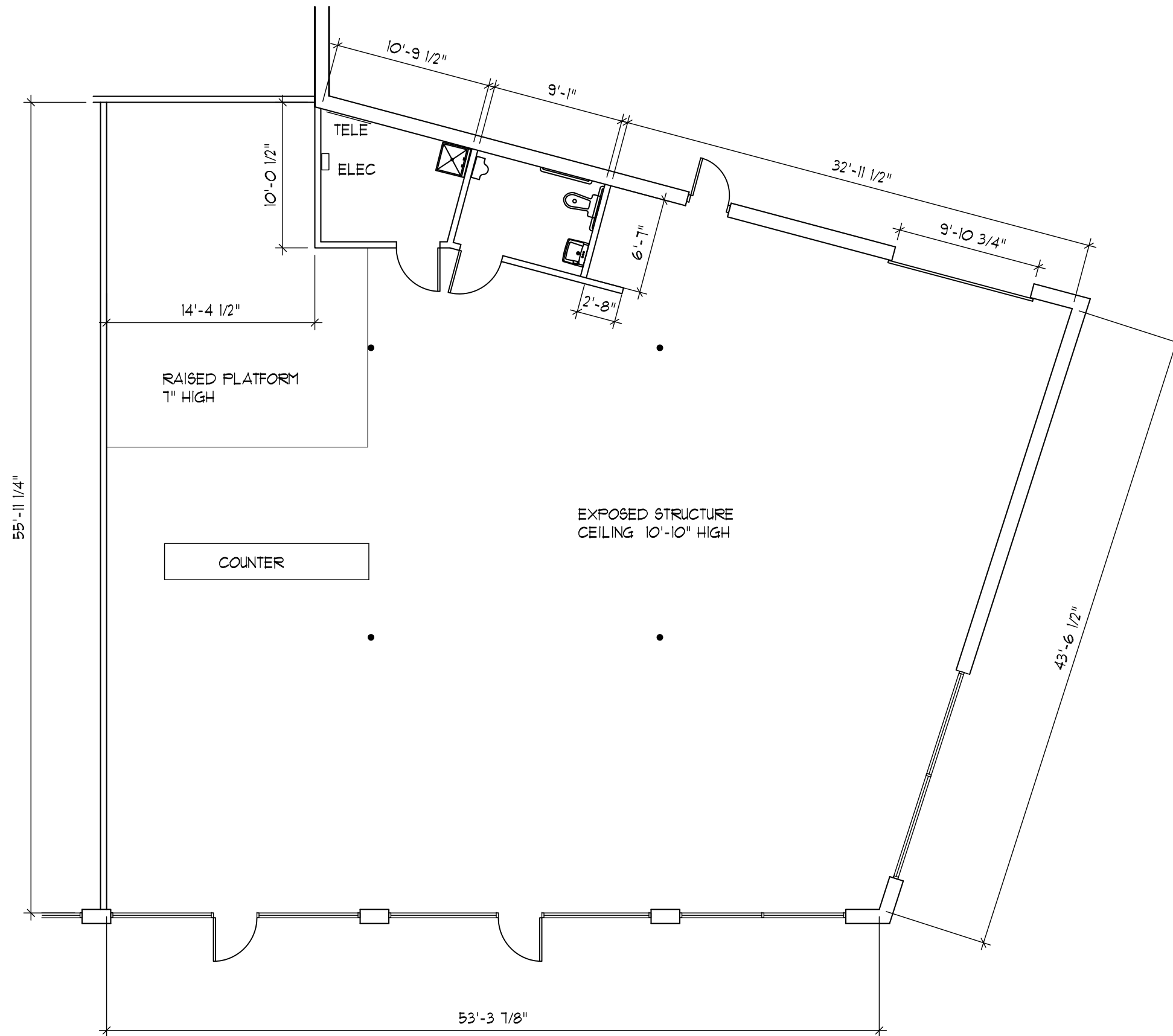
1 SUITE 100 EXISTING PLAN - 3195 SQ. FT. (APPROX) 1/8" = 1'-0"
