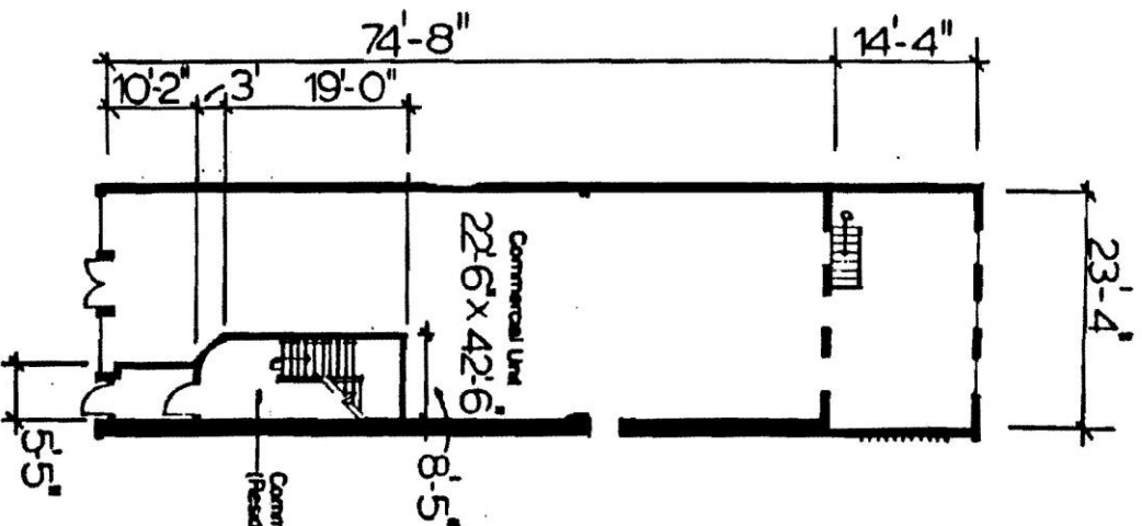
First Floor
