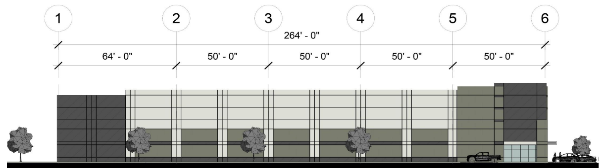
SIDE ELEVATION
