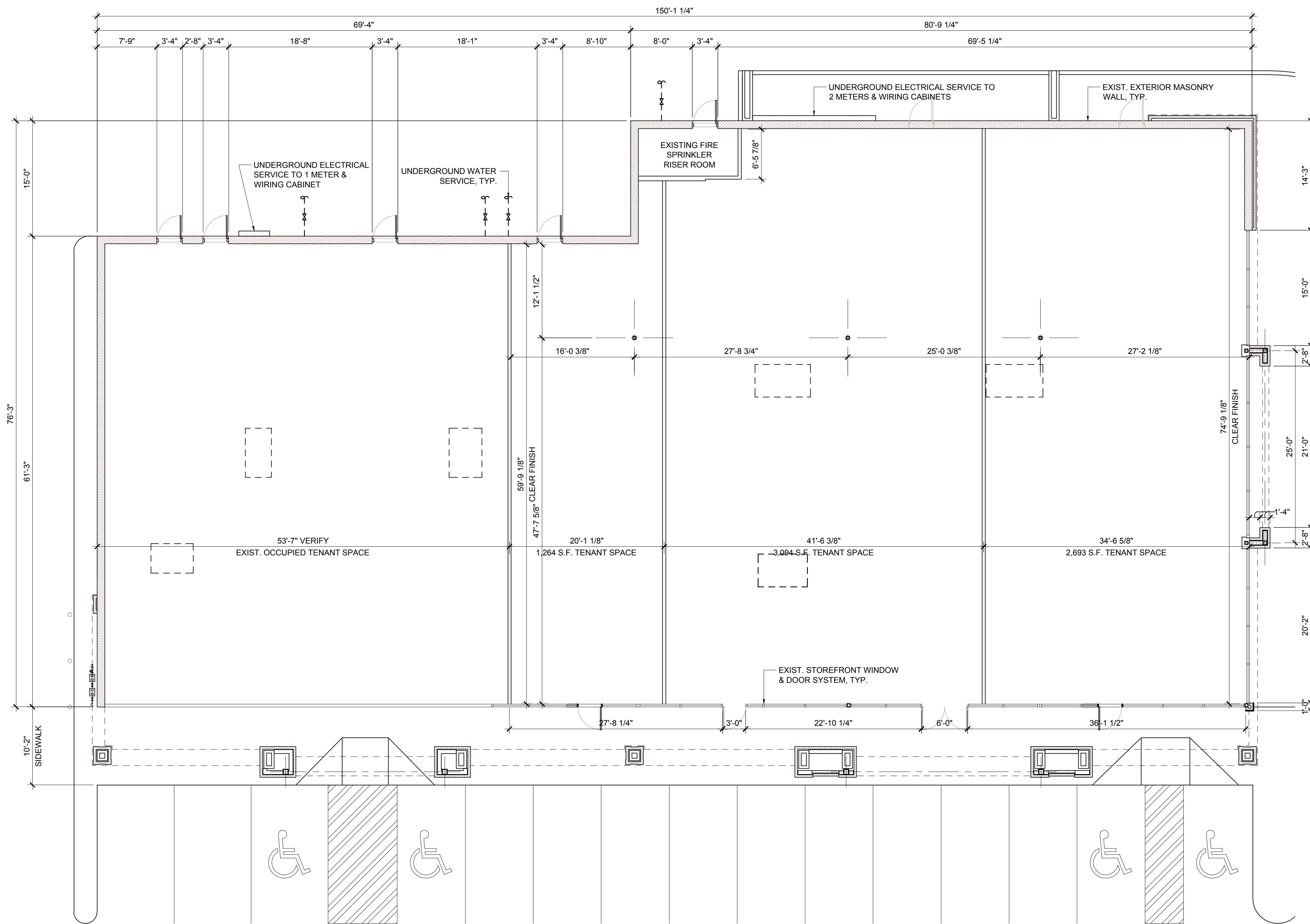
1 SOUTH OUTLOT BUILDING FLOOR PLAN PRA1.0 SCALE: 1/8" = 1'-0" NORTH
