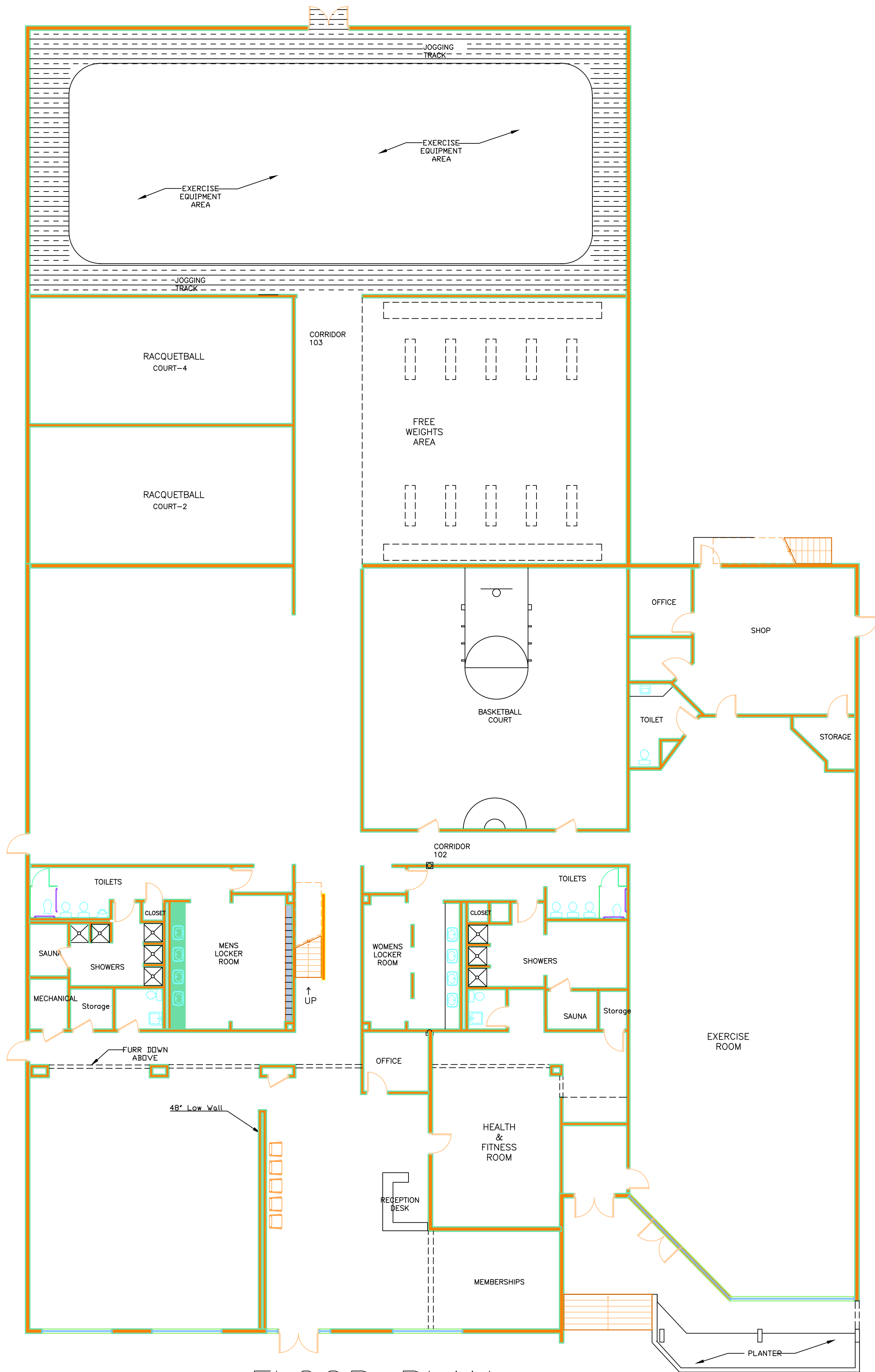
FLOOR PLAN LOWER LEVEL
