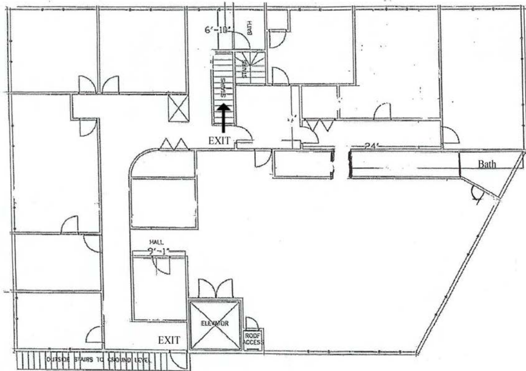
2nd Floor
