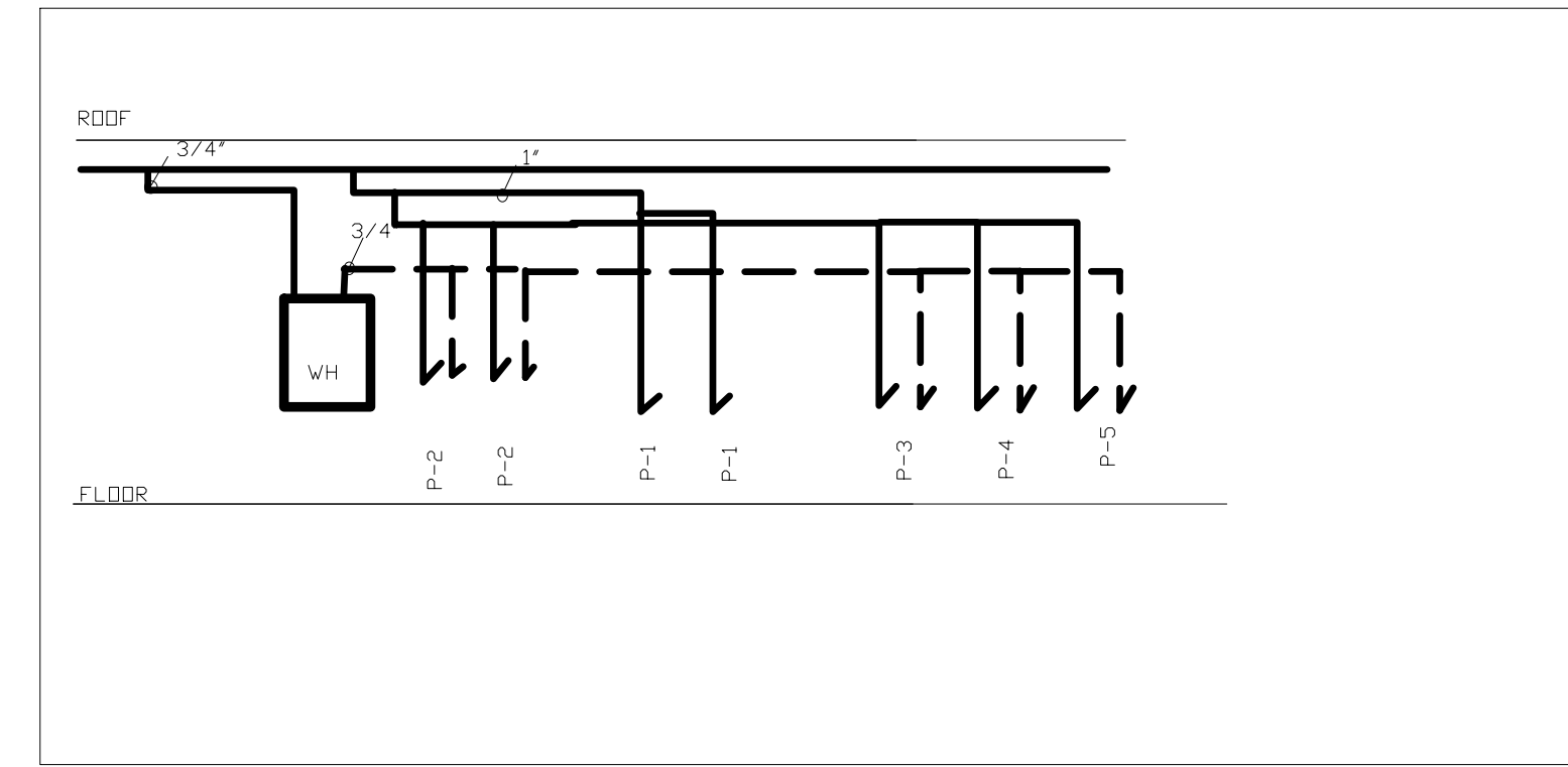
2 DOMESTIC WATER RISER DIAGRAM NO SCALE
