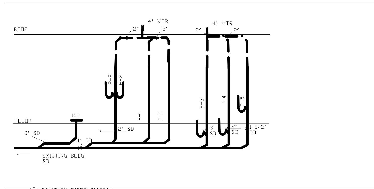
1 SANITARY RISER DIAGRAM NO SCALE
