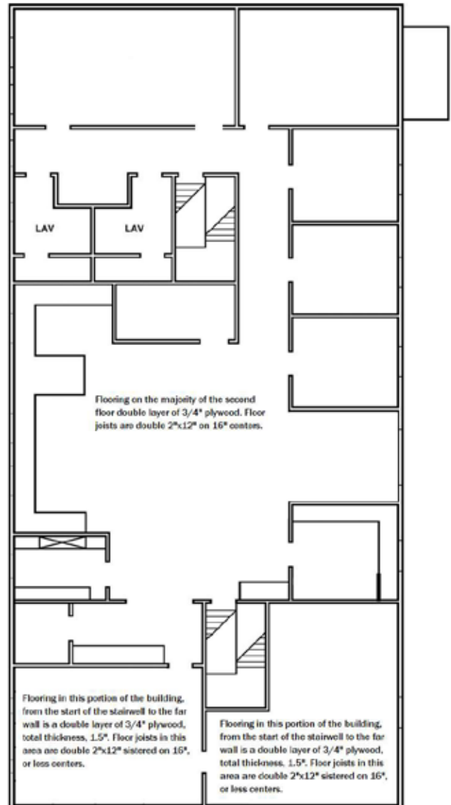
SECOND FLOOR SCHEMATIC
