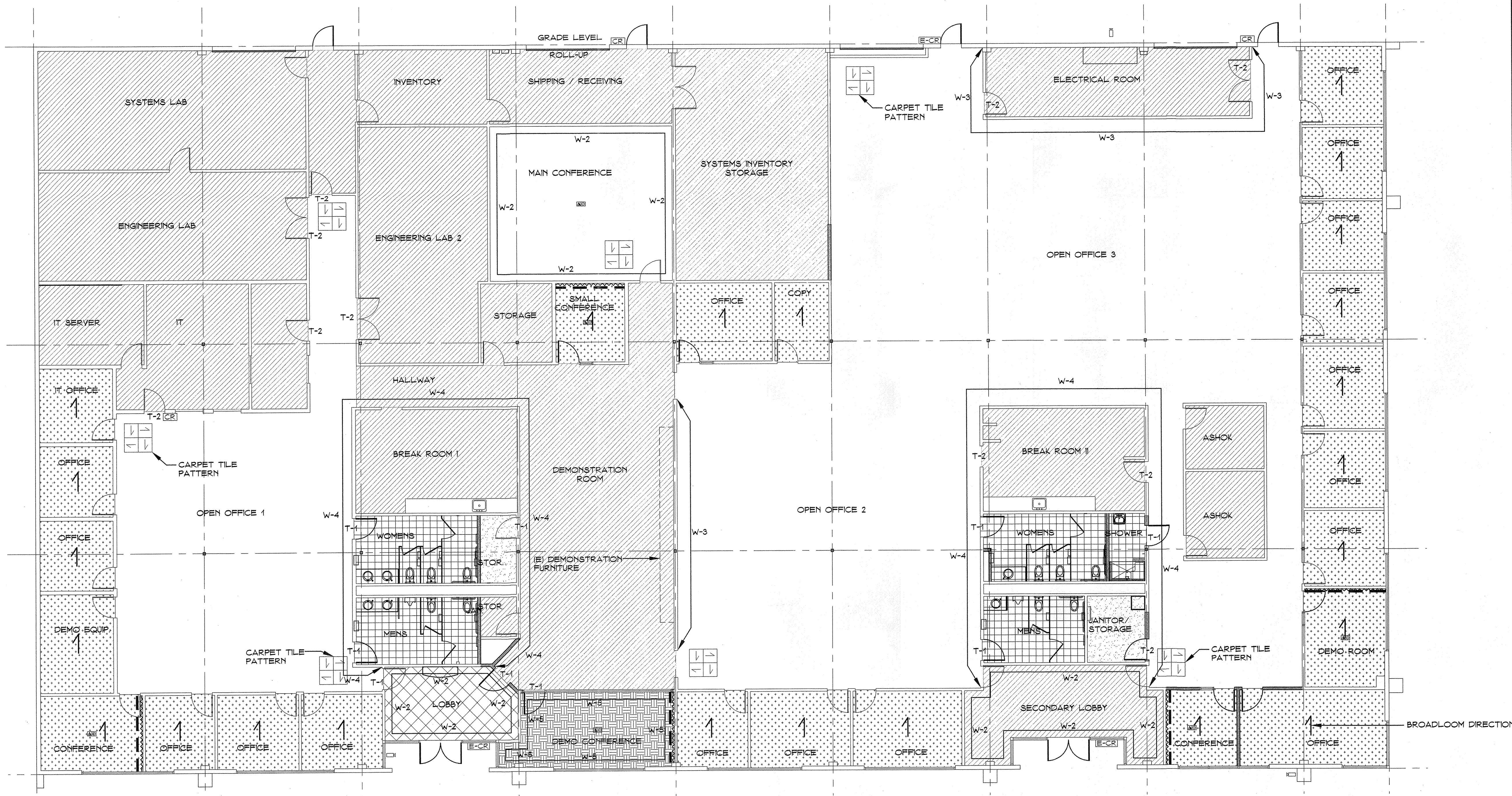
Finish Plan 1/8" = 1'-0" NORTH
