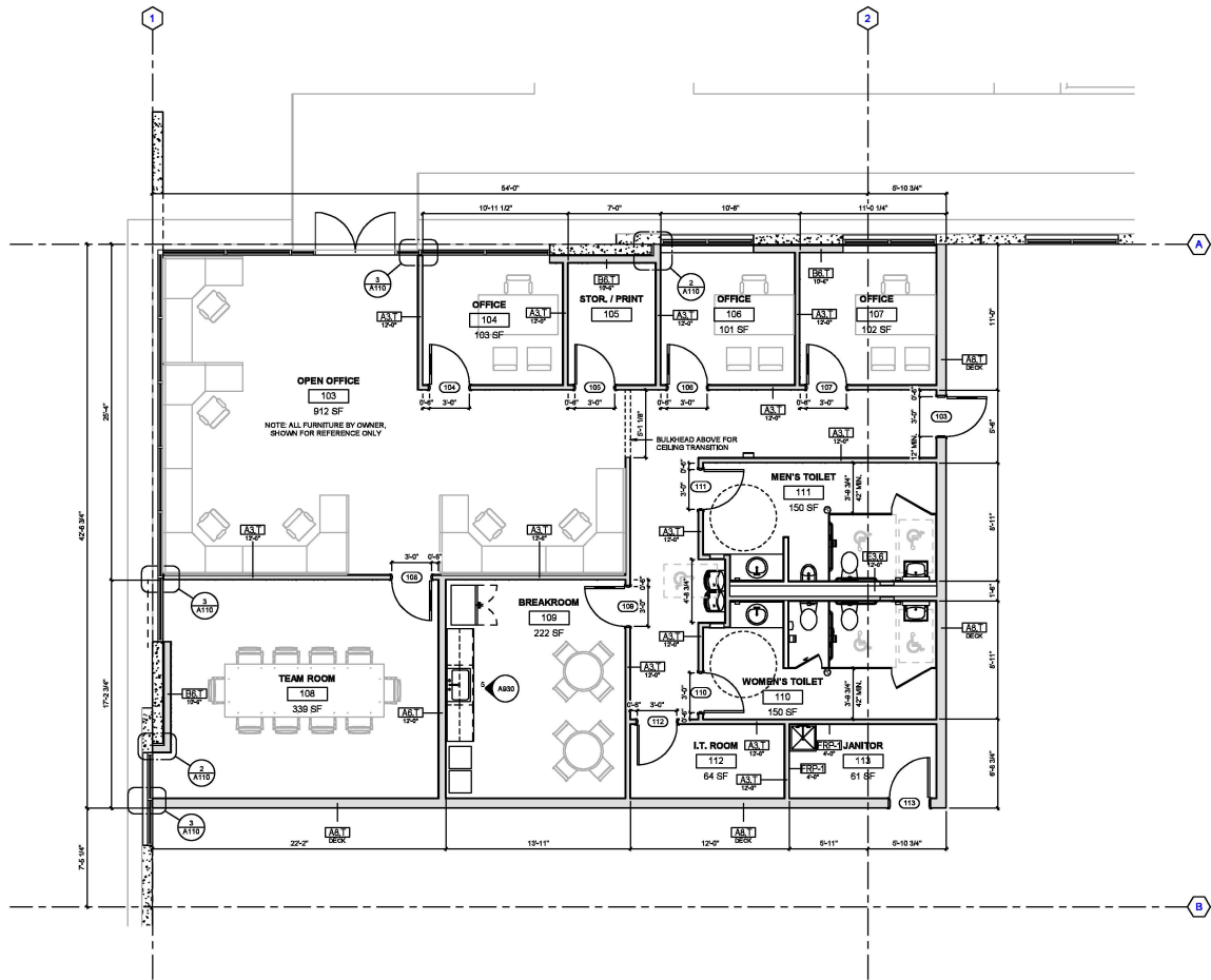
1 OFFICE PLAN SCALE: 1/4" = 1'-0"
