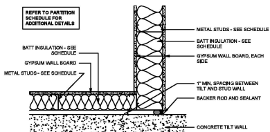
2 PARTITION TO FURRING AT TILT SCALE: 1 1/2" = 1'-0" | ARCO: 131.02
