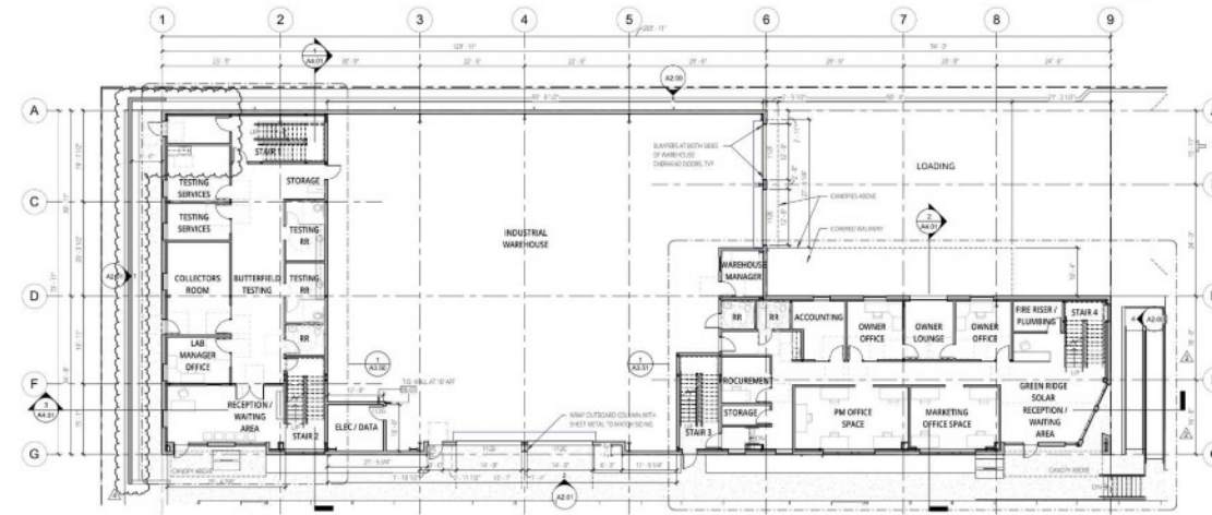
1 GROUND FLOOR PLAN
