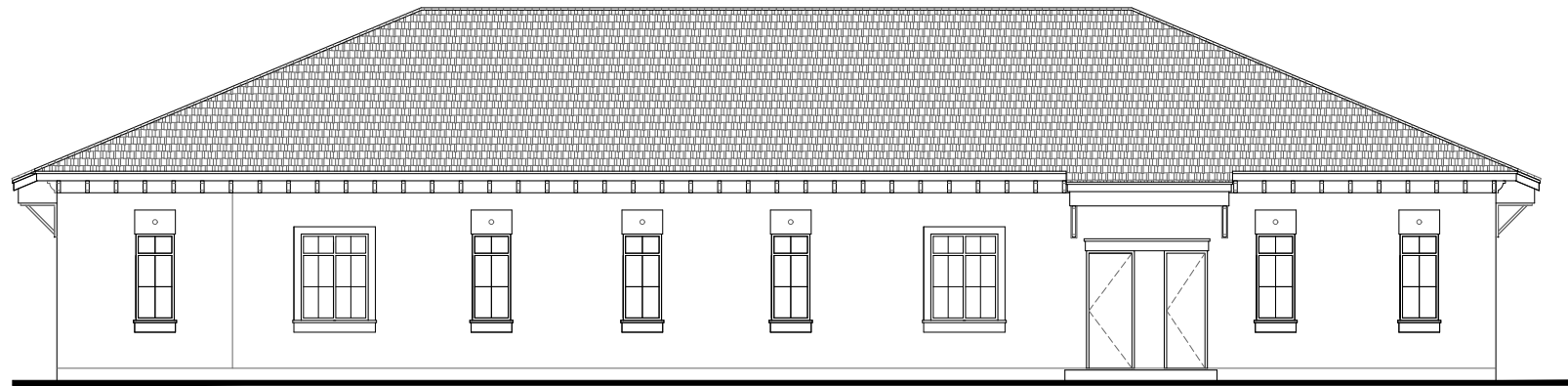
REAR (SOUTH) ELEVATION/ BUILDING 'B'
