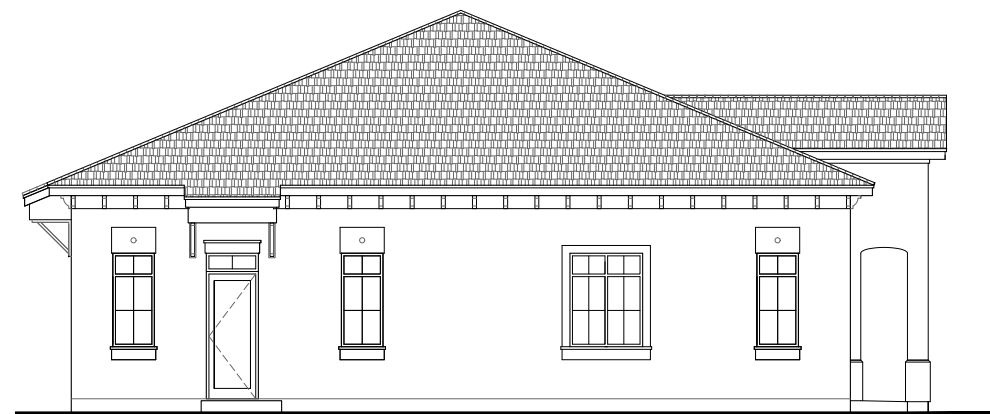
LEFT SIDE (EAST) ELEVATION/ BUILDING 'B'
