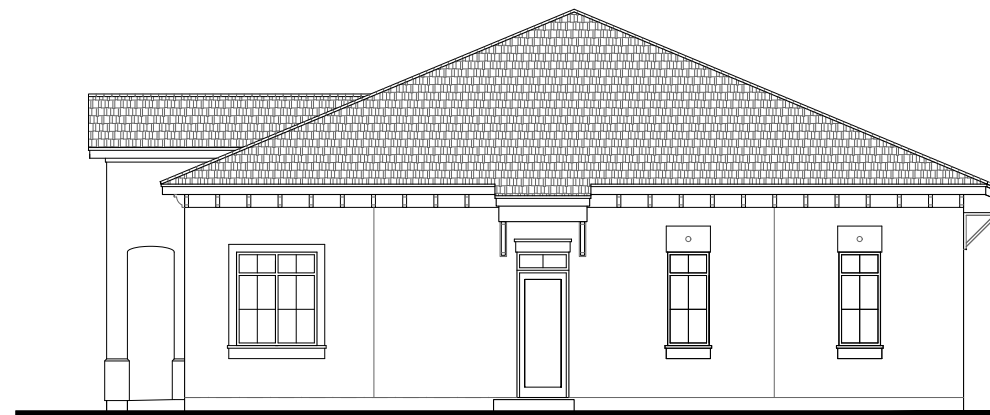
RIGHT SIDE (WEST) ELEVATION/ BUILDING 'B'
