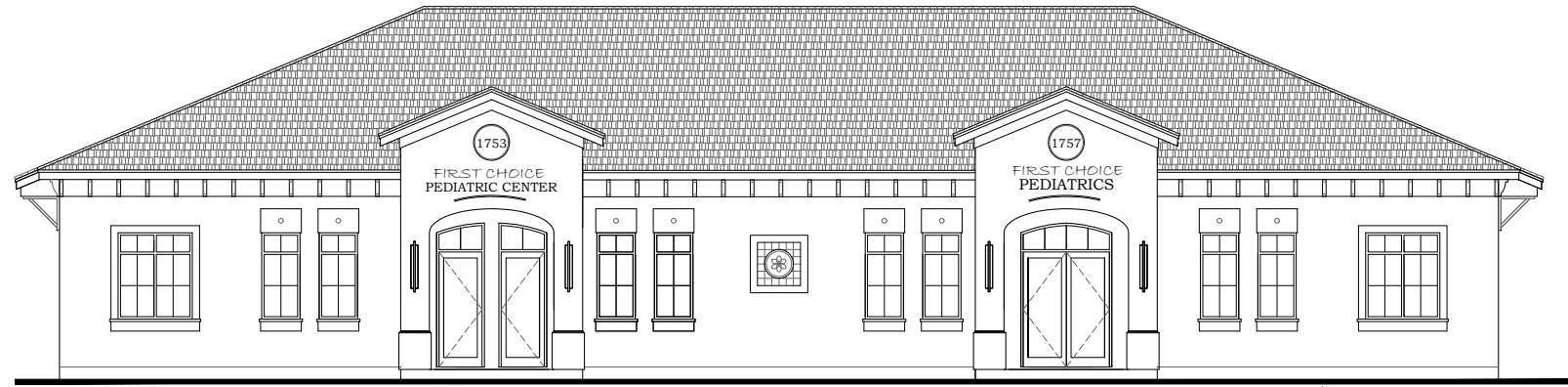
FRONT (NORTH) ELEVATION/ BUILDING 'B'
