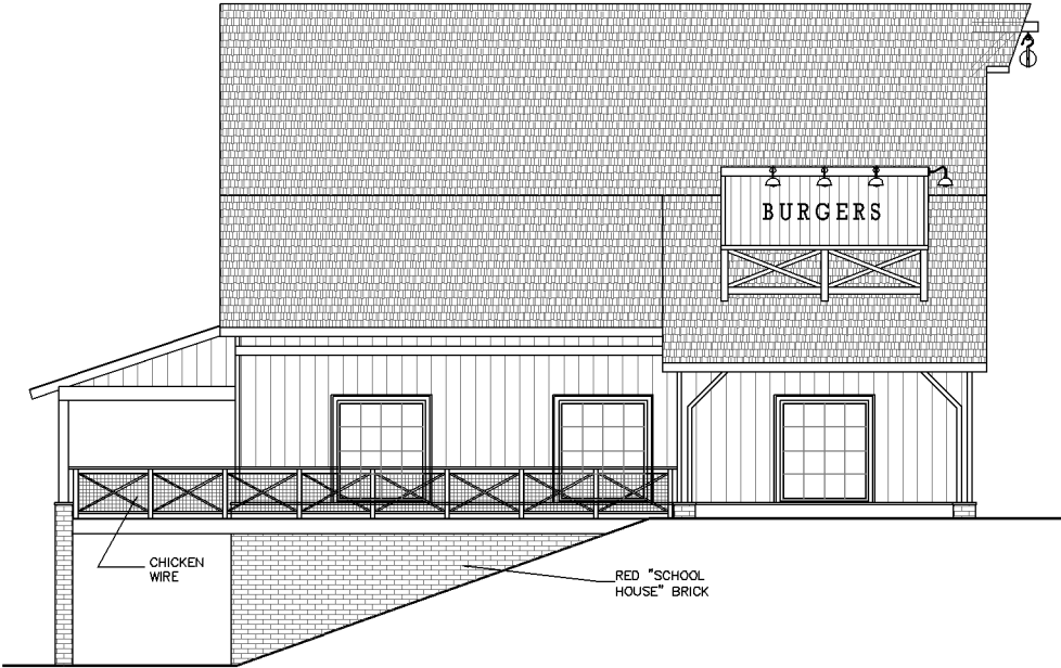
PROPOSED "WILEY MARKET" SITE RESTAURANT BUILDING DESIGN
