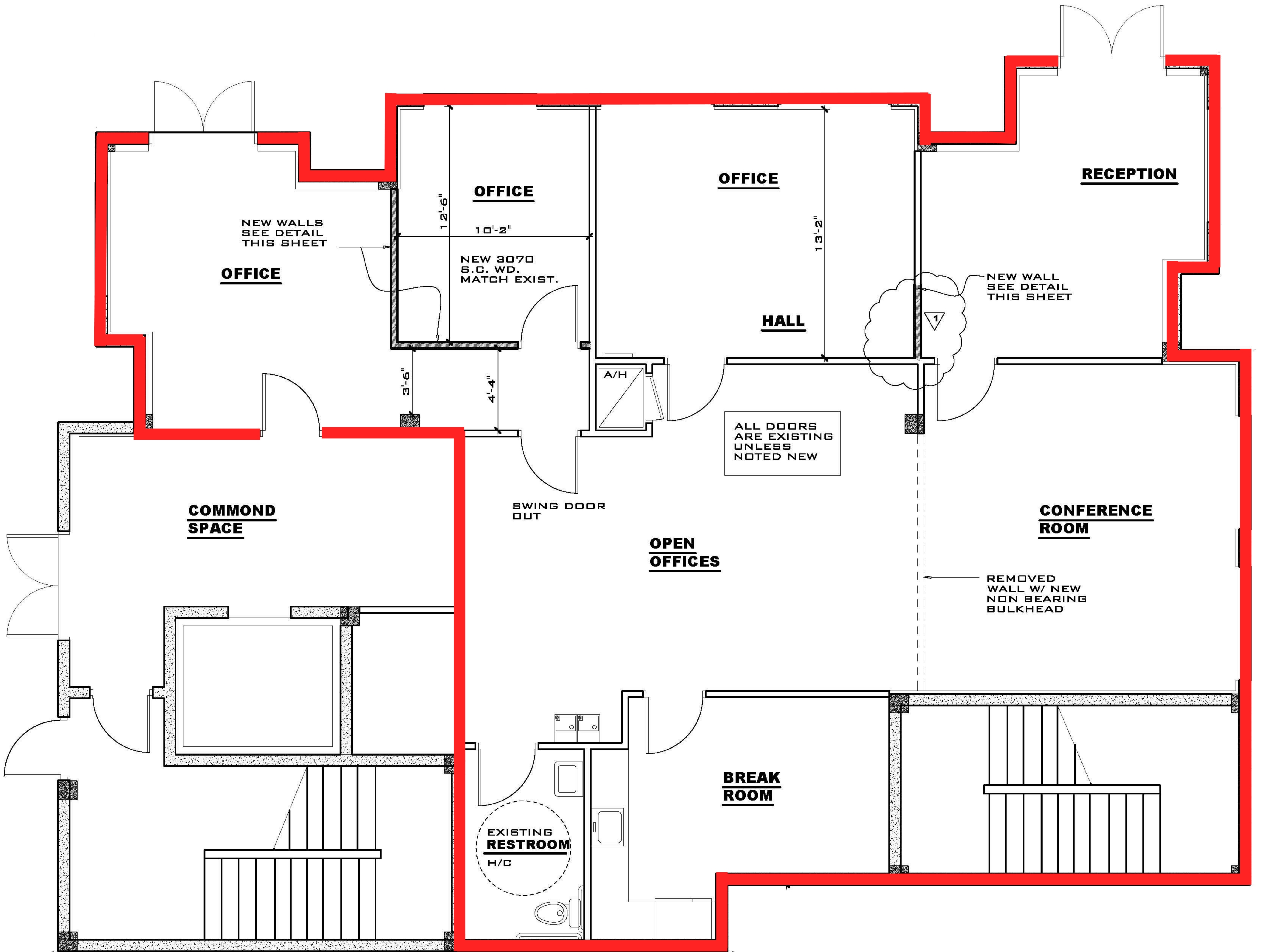
1st Floor - Floor Plan
