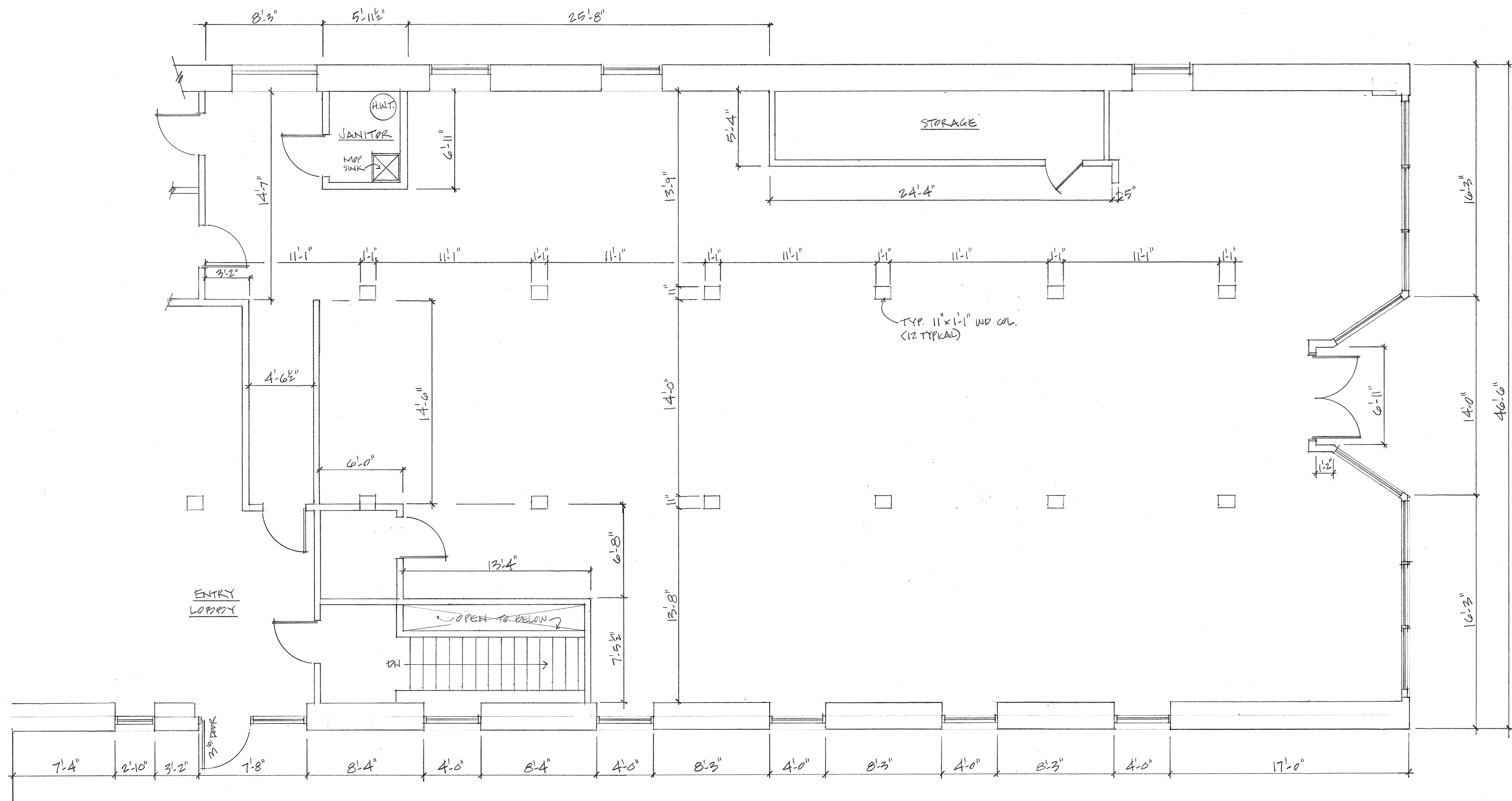
MAIN FLOOR PLAN 3,762.7 S.F. 1/4" = 1'-0"
