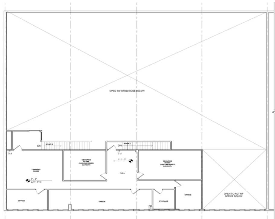
2nd Floor/Mezzanine
