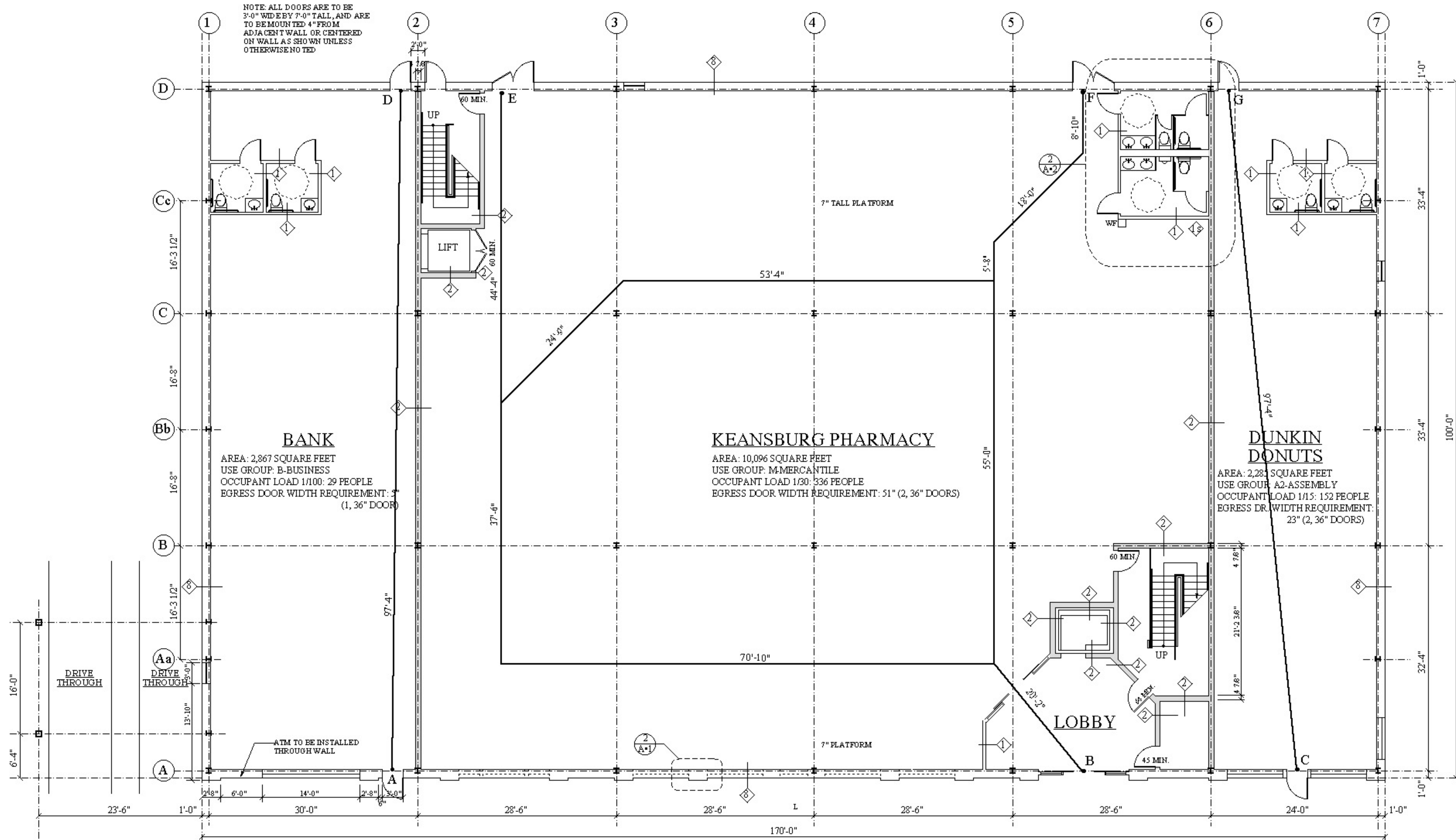
1 GROUND FLOOR PLAN SCALE: 1/8" = 1'-0"
