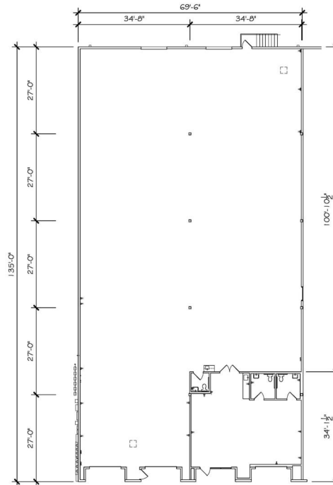
EXISTING PLAN 9-4-24 1/16" = 1'-0" 762 ISOM RD. - 9,450 sq.ft.
