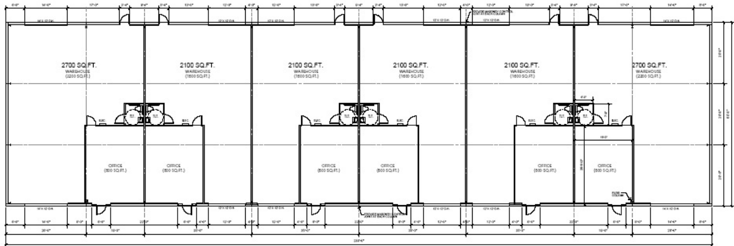
FLOOR PLAN 13,800 SQ.FT. TOTAL B & S1 OCCUPANCY - TYPE IIN - NON-SPRINKLERED ONE STORY
