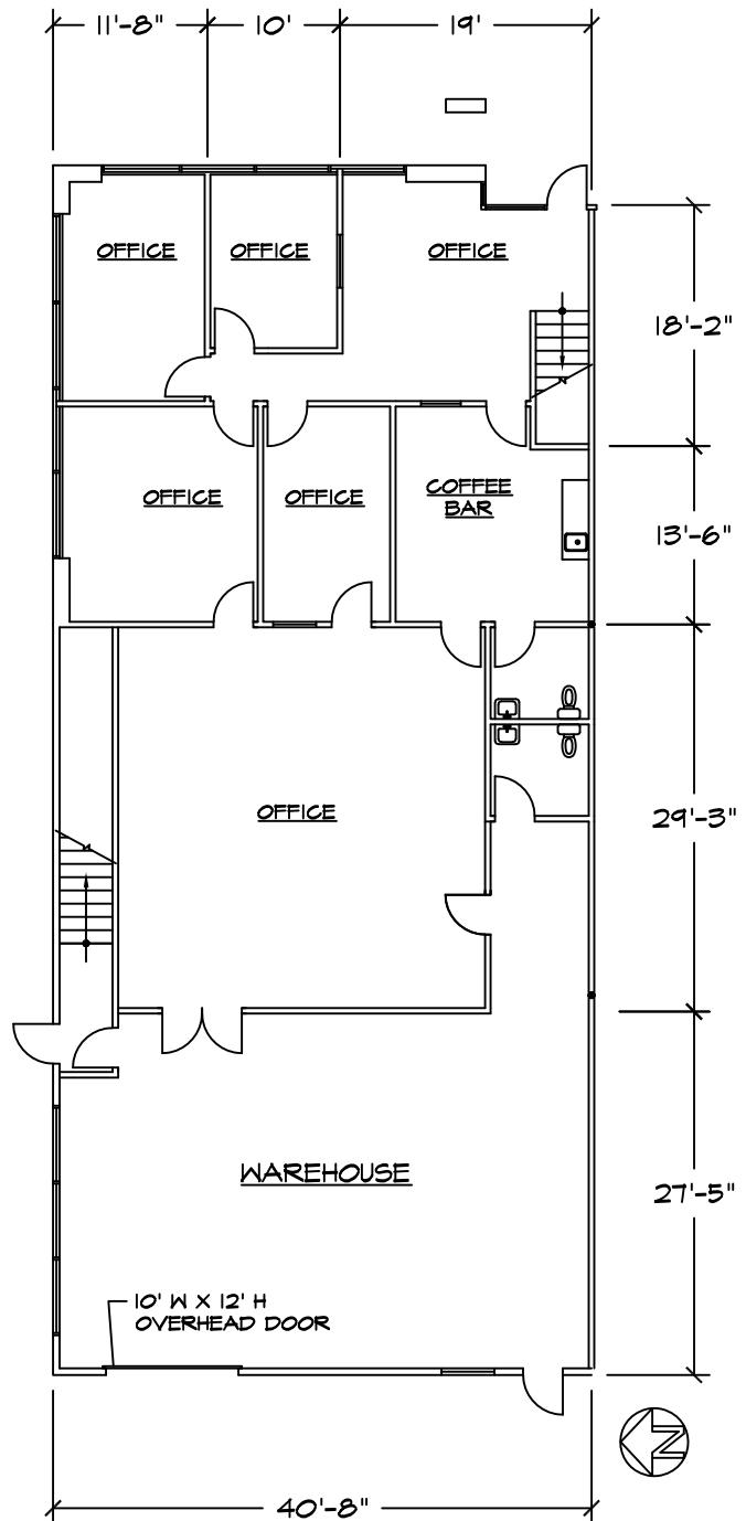
FIRST FLOOR
