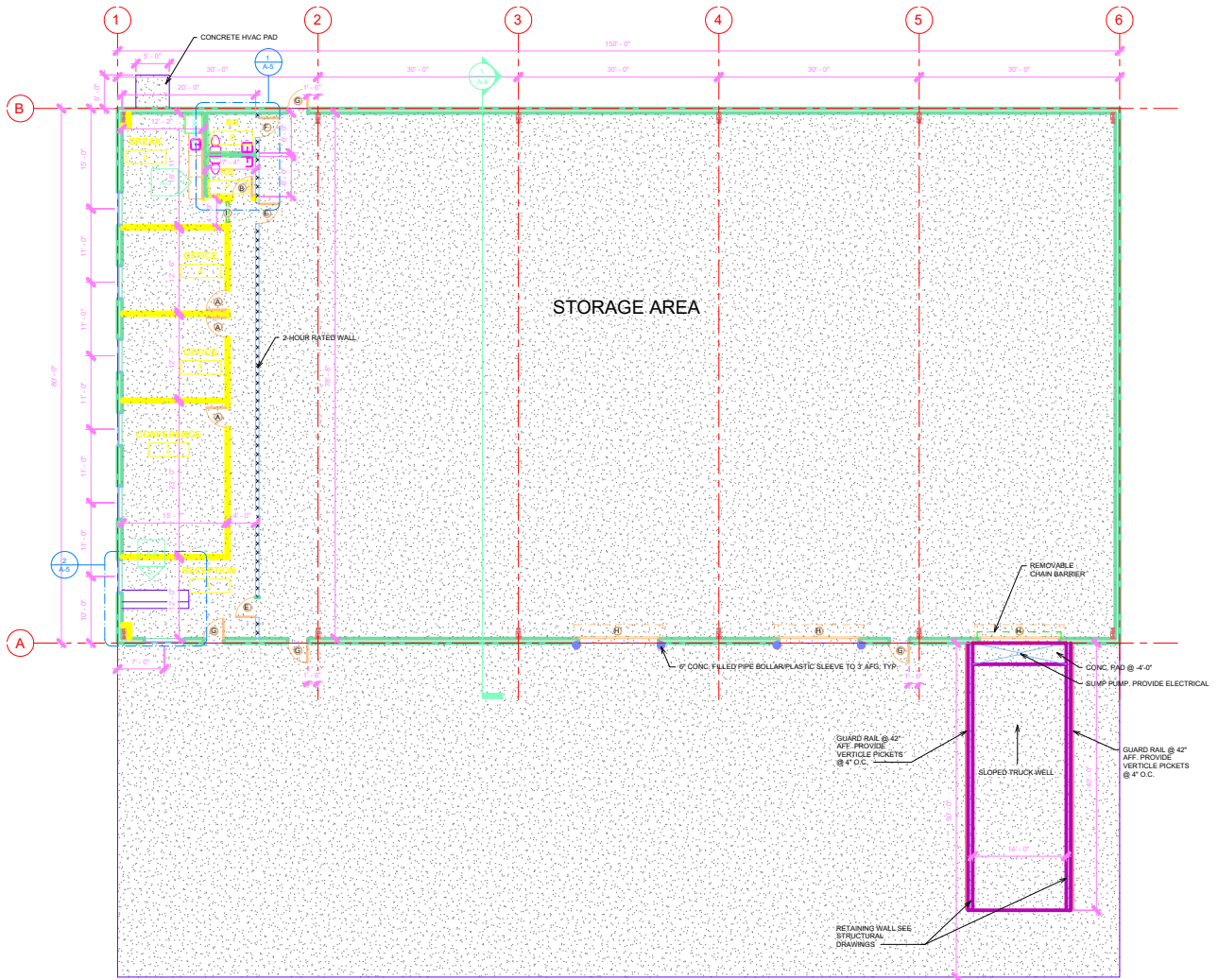
FLOOR PLAN 1/8" = 1'-0"
