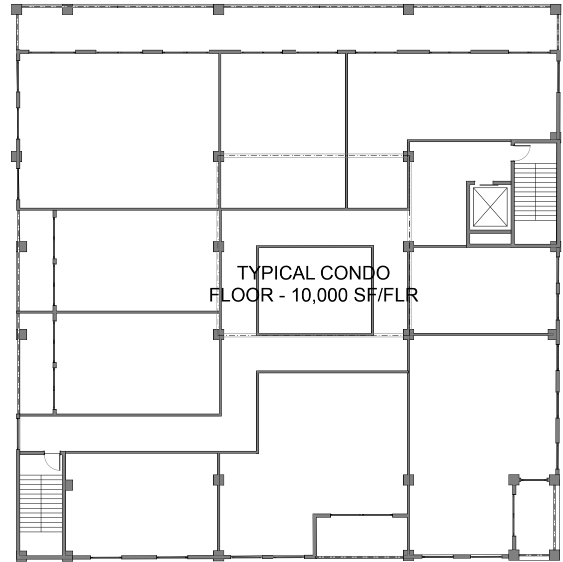
CONDO BUILDING - SECOND AND THIRD FLOOR PLAN 9 UNITS/FLOOR ( 500-1200SF)
