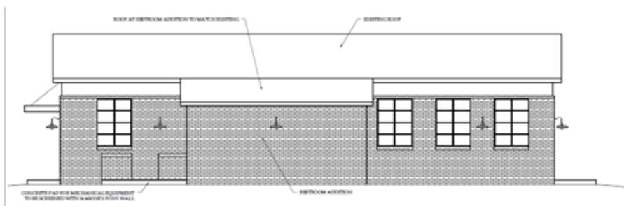
South Elevation
