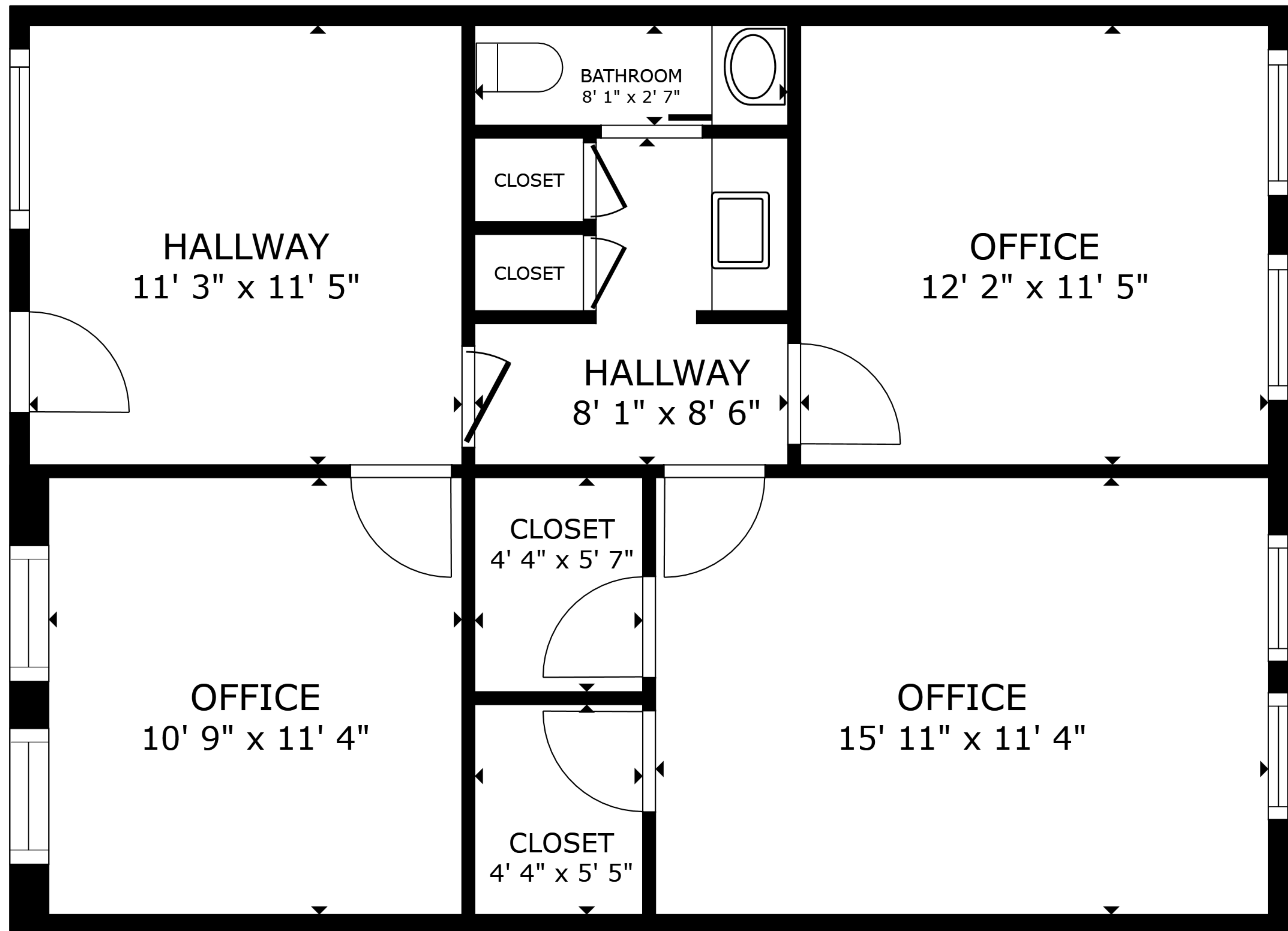
FLOOR PLAN
