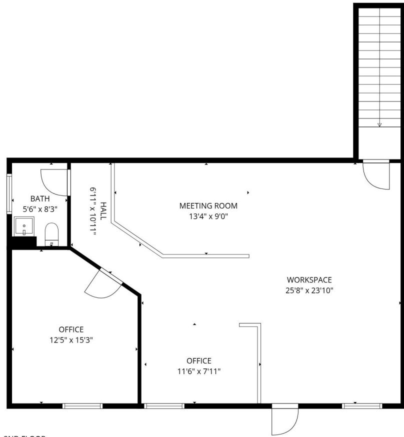
2ND FLOOR
