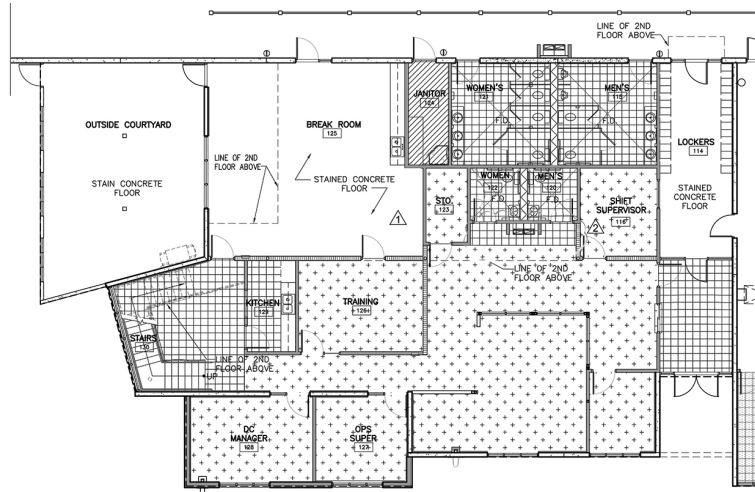
1ST FLOOR - MAIN OFFICE (±5,843 SF)
