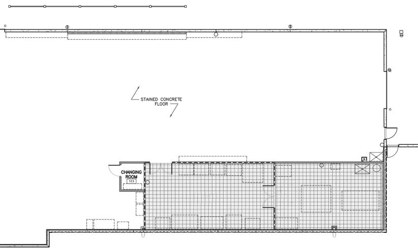
1ST FLOOR - QC LAB (±5,686 SF)
