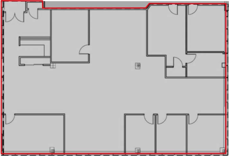
PART 4TH FLOOR PLAN: 4,495 SF
