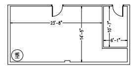
SECOND FLOOR (MEZZANINE ADJACENT) 484 SF
