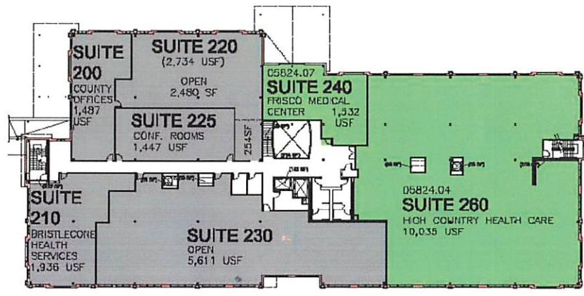
2 SECOND FLOOR PLAN 1/4" = 1'-0"
