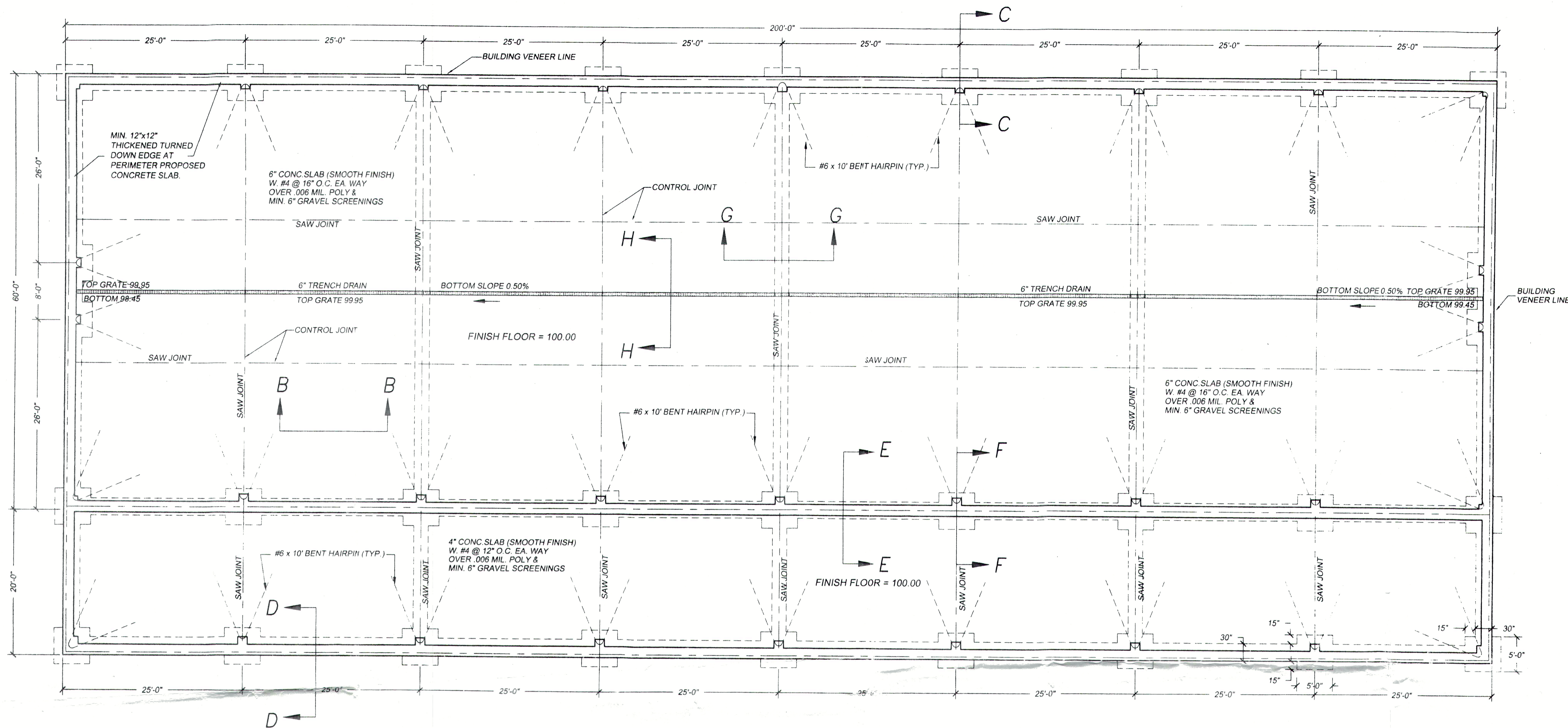
FOUNDATION PLAN SCALE: 1/8" = 1'
