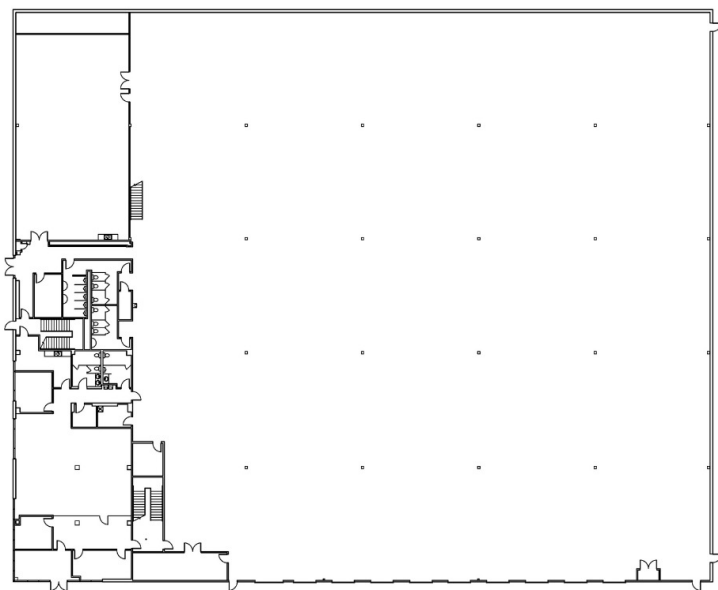
1 FLOOR PLAN - FIRST FLOOR NTS
