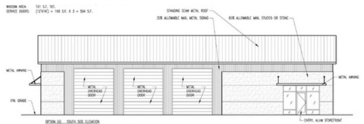
4 SOUTH ELEVATION 1/8" = 1'-0"
