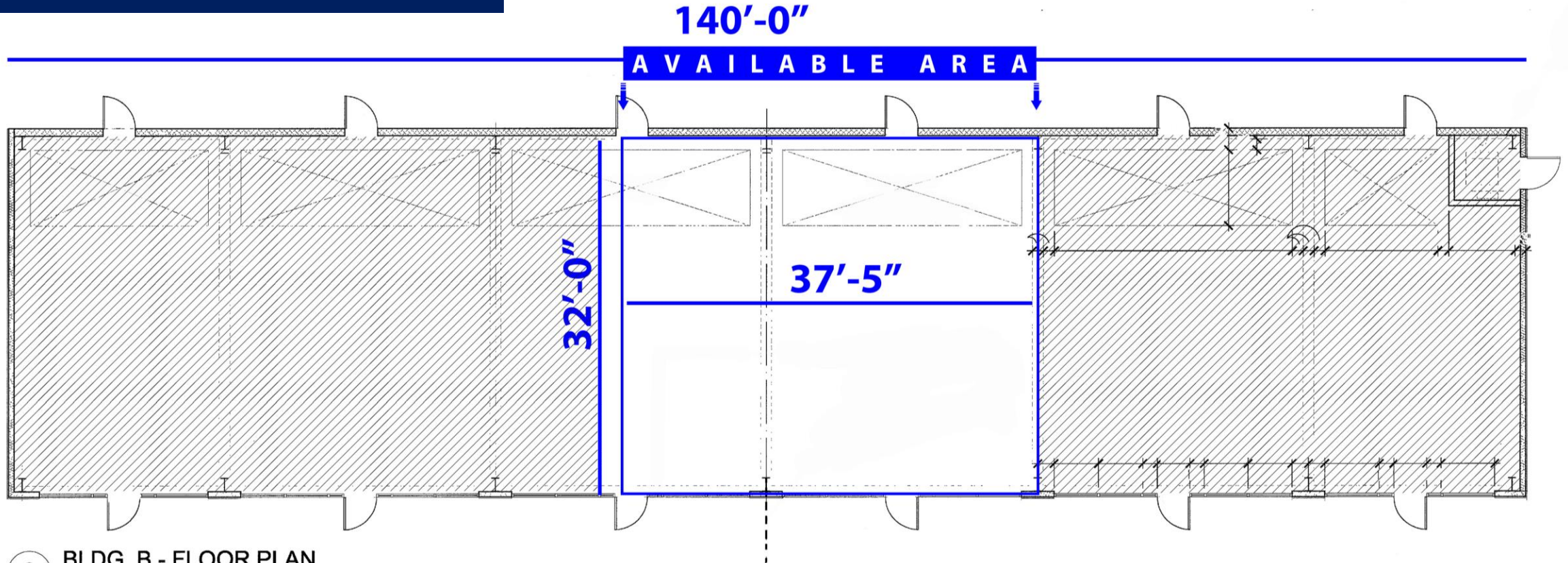
2 BLDG. B - FLOOR PLAN 1/8" = 1'-0"
