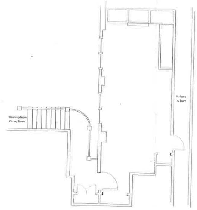
Mezzanine Plan Scale 3/8" = 1'-0"
