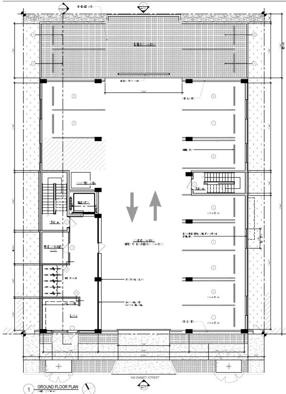
166-170 Emmet Street Ground Floor Plan
