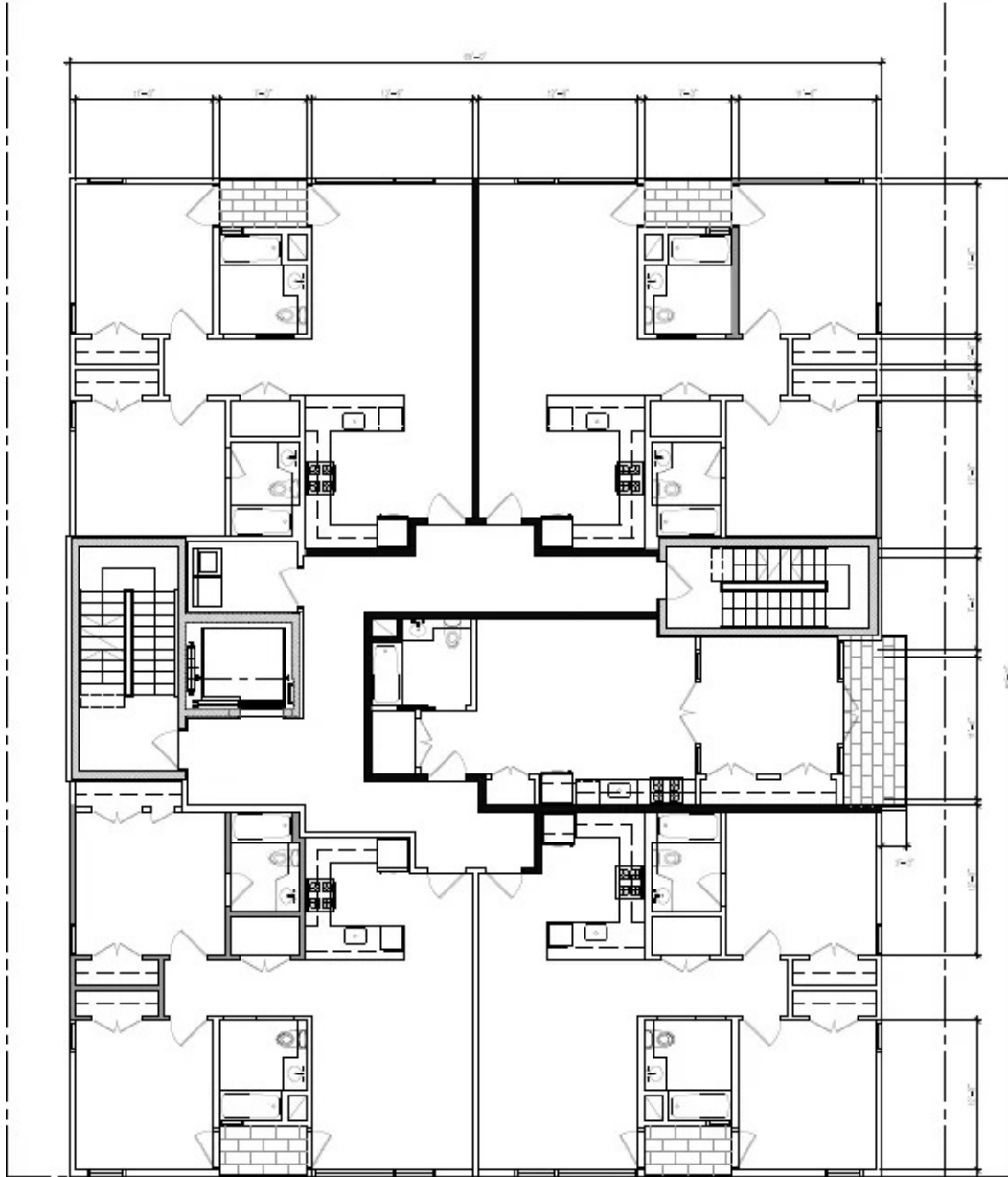
166-170 Emmet Street Typical Floor Plan 2-4
